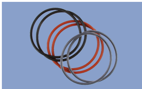
Closure O-Rings: Nitrile, VITON® and TEFLON® encapsulated VITON®, Silicone, EPDM
